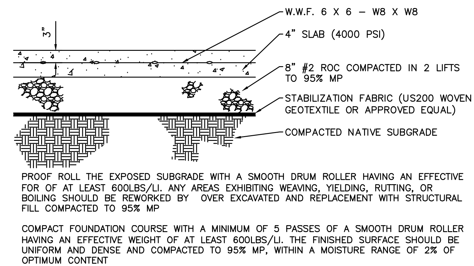
CONCRETE SLAB NTS
